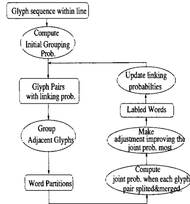
Figure 1. Overview of the word segmentation algorithm
